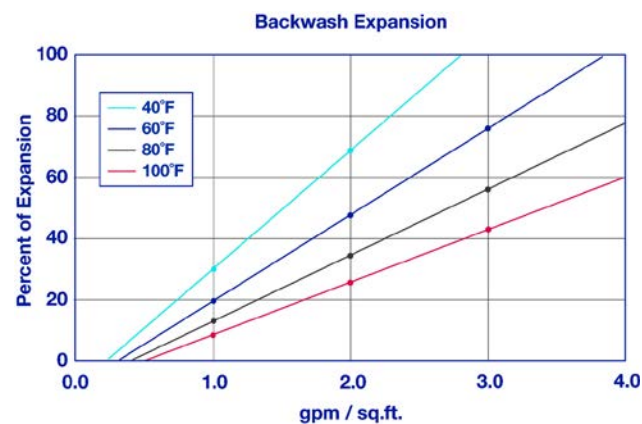
The graph above shows the expansion characteristics of ResinTech SBG1-OH-SC as a function of flow rate at various temperatures.
