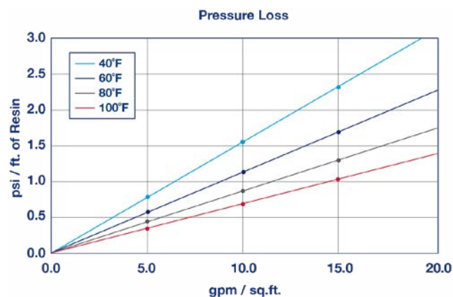
The graph above shows the expected pressure loss of ResinTech SBG1-OH-SC per foot of bed depth as a function of flow rate at various temperatures.
