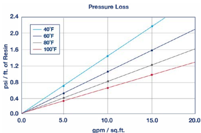
The graph above shows the expected pressure loss of ResinTech CG10-BL-HP per foot of bed depth as a function of flow rate at various temperatures.
