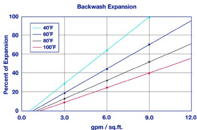
The graph above shows the expansion characteristics of ResinTech CG10-BL-HP as a function of flow rate at various temperatures.
