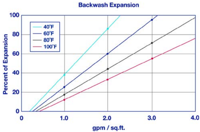
The graph above shows the expansion characteristics of ResinTech SBMP1-OH as a function of flow rate at various temperatures.
