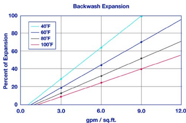
The graph above shows the expansion characteristics of ResinTech CG10-BL-UPS as a function of flow rate at various temperatures.
