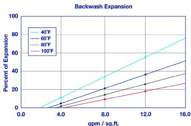
The graph above shows the expansion characteristics of ResinTech AGC-40 CA as a function of flow rate at various temperatures.
