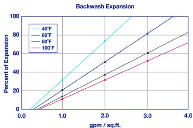
The graph above shows the expansion characteristics of ResinTech SBACR-MP-HP as a function of flow rate at various temperatures.
