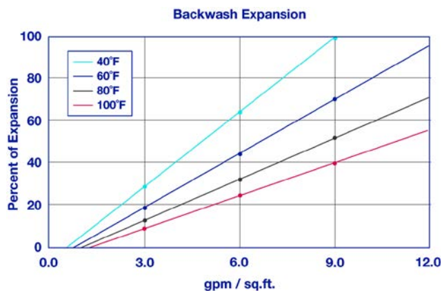
The graph above shows the expansion characteristics of ResinTech CG10-NA as a function of flow rate at various temperatures.
