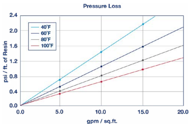
The graph above shows the expected pressure loss of ResinTech CG10-NA per foot of bed depth as a function of flow rate at various temperatures.
