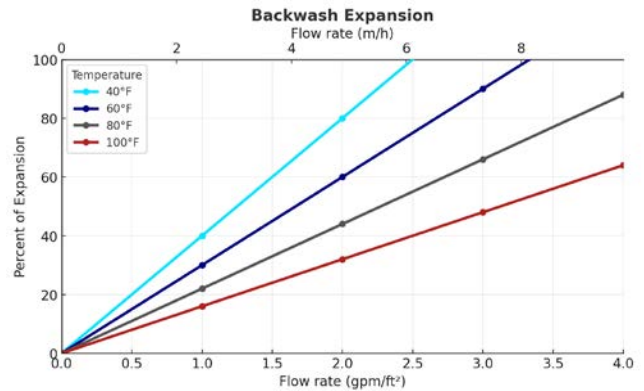
The graph above shows the expansion characteristics of ResinTech SBG1P-OH-SC as a function of flow rate at various temperatures.
