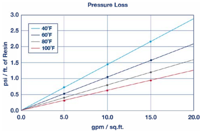
The graph above shows the expected pressure loss of ResinTech SBG1P-OH-SC per foot of bed depth as a function of flow rate at various temperatures.
