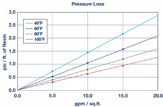
The graph above shows the expected pressure loss of ResinTech SBG1P-OH-ULTRA per foot of bed depth as a function of flow rate at various temperatures.
