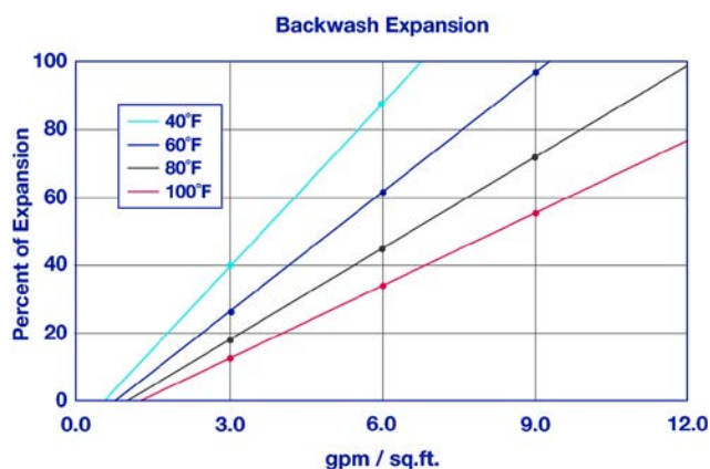
The graph above shows the expansion characteristics of ResinTech CG8-H as a function of flow rate at various temperatures.
