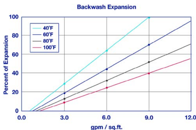
The graph above shows the expansion characteristics of ResinTech CG10-H-BL as a function of flow rate at various temperatures.
