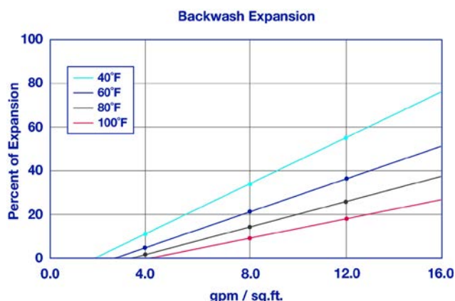
The graph above shows the expansion characteristics of ResinTech AGC-40 X as a function of flow rate at various temperatures.
