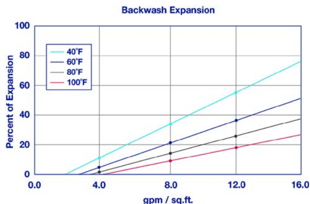
The graph above shows the expansion characteristics of ResinTech AGC40-CTR as a function of flow rate at various temperatures.
