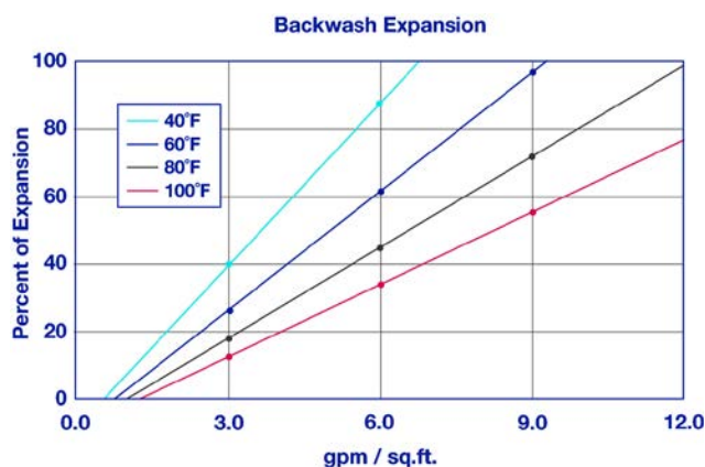
The graph above shows the expansion characteristics of ResinTech CNS-C as a function of flow rate at various temperatures.
