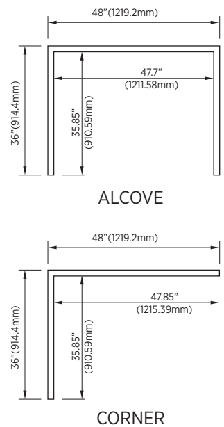
TOP VIEW (ASSEMBLED)
