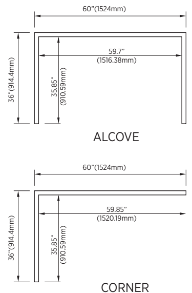
TOP VIEW (ASSEMBLED)
