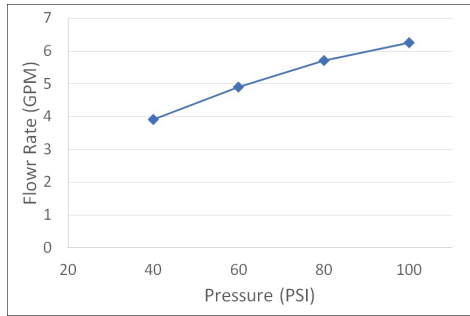
V-2300B-EP90U Flow Rate (GPM) Vs Pressure (PSI) For Tub Port*
