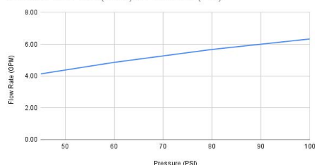
V-2600B Flow Rate(GPM) Vs Pressure (PSI)
