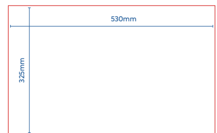
Required cut-out for the elevator panel
